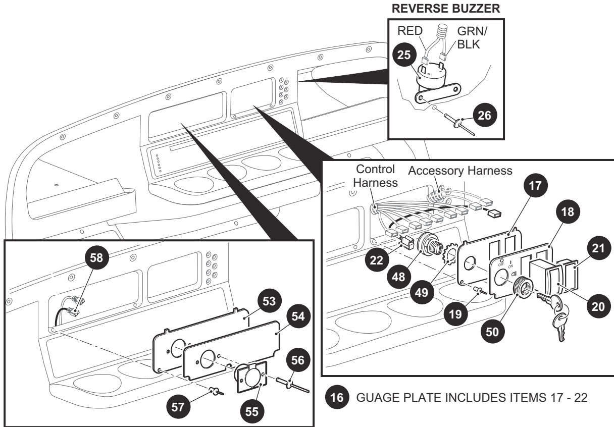
CONSOLE INSERT PLATE (WITH POWER OUTLET SHOWN)
