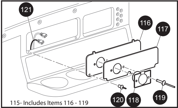
CONSOLE INSERT PLATE (WITH POWER OUTLET SHOWN)
