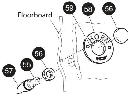
HORN BUTTON
