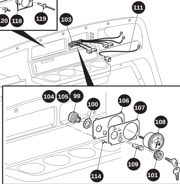
KEY SWITCH, INDICATOR LIGHT(S), AND FUEL GAUGE
