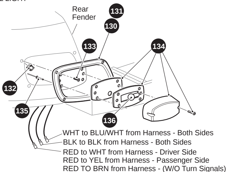
TAIL LIGHT
