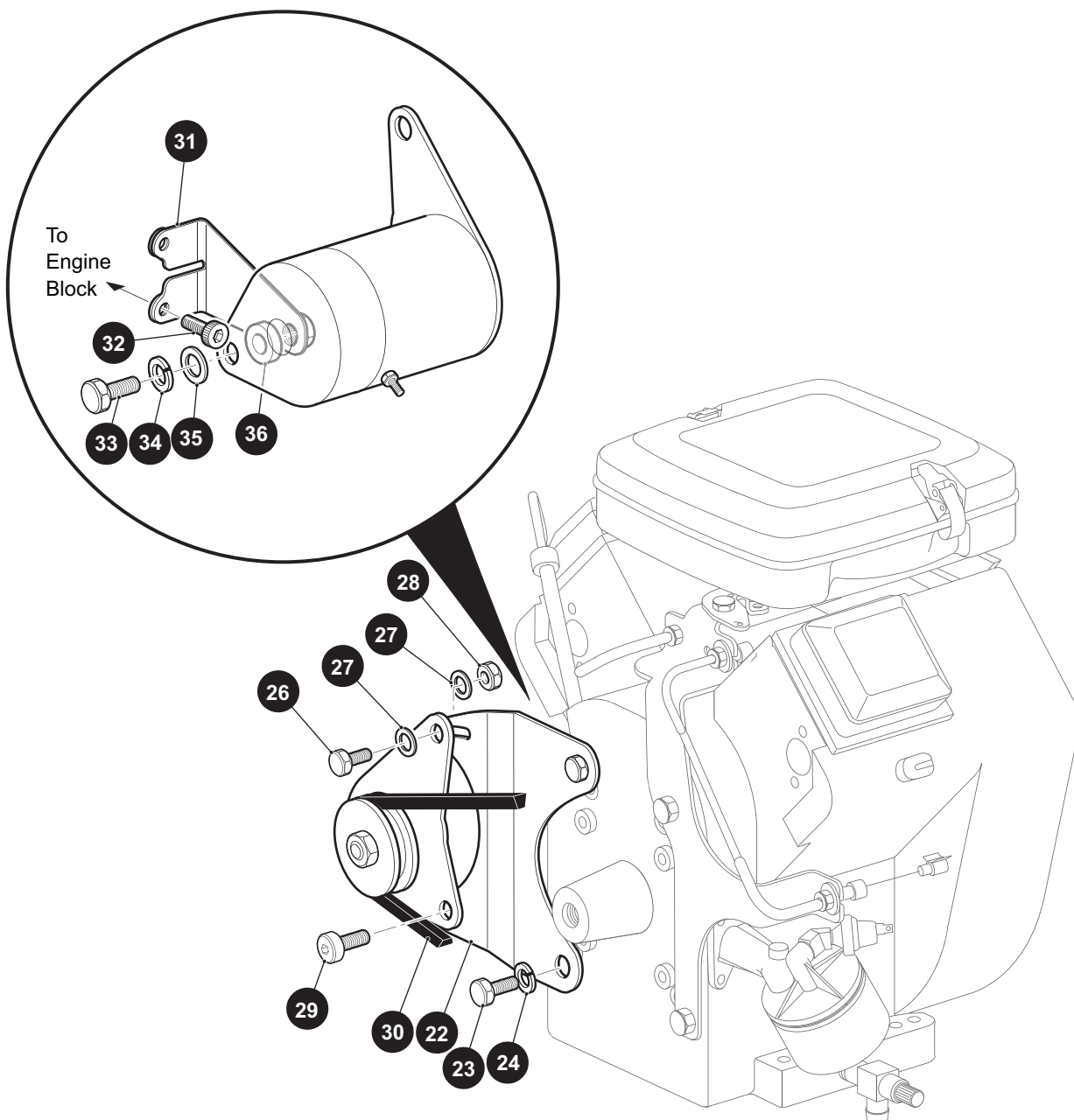
REAR VIEW
