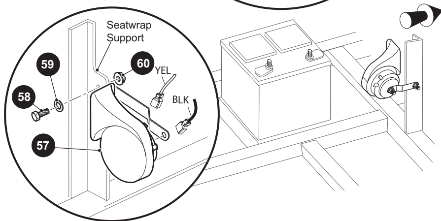
HORN
