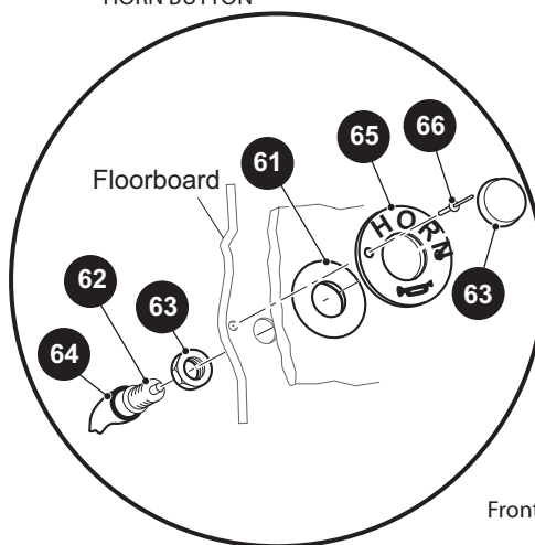
HORN BUTTON
