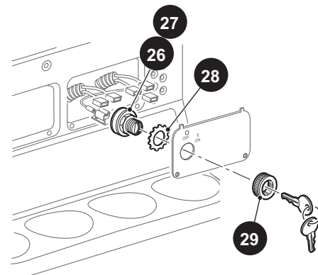
KEY SWITCH AND KEY SET
