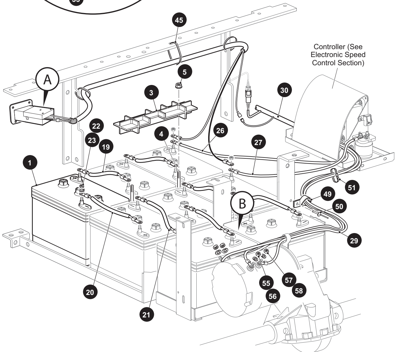
31 CHARGER RECEPTACLE ASSEMBLY Includes Items 32 - 40
