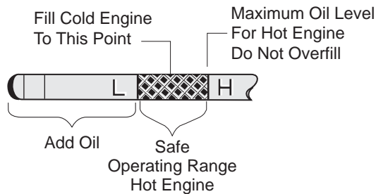
Check Oil Level on Dipstick
