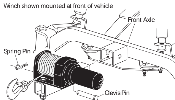
Winch Mounted to Vehicle
