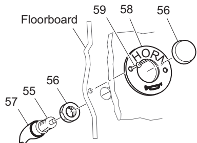
HORN BUTTON
