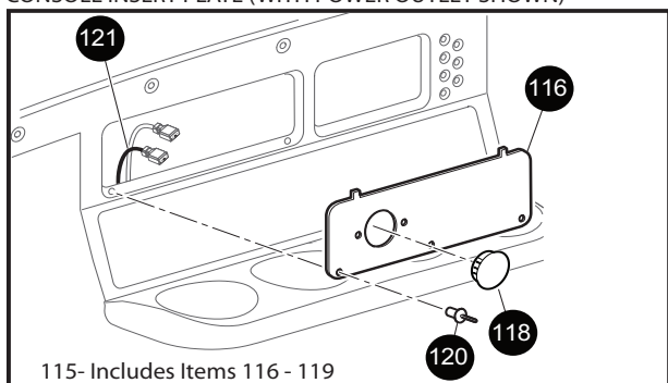
CONSOLE INSERT PLATE (WITH POWER OUTLET SHOWN)
