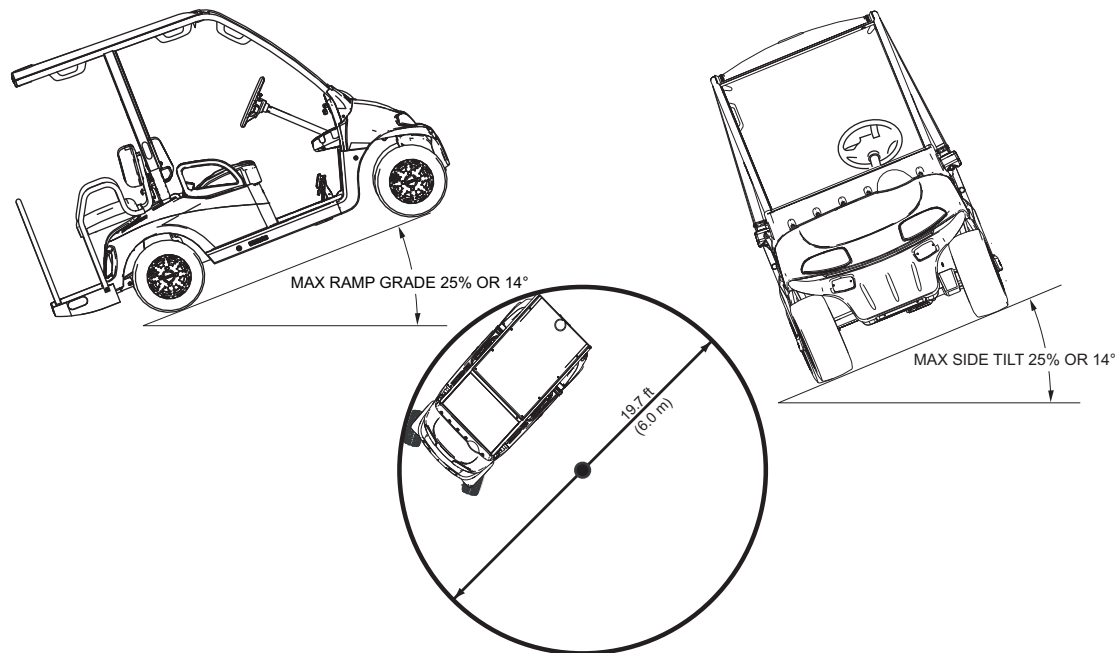
Fig. 5 Vehicle Incline Specifications and Turning Diameter
