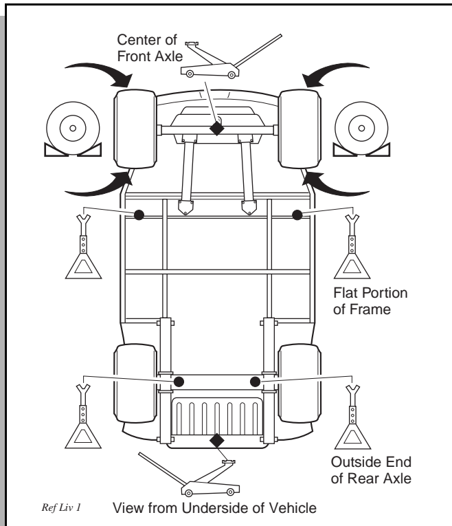
Fig. 14 Lifting the Vehicle
