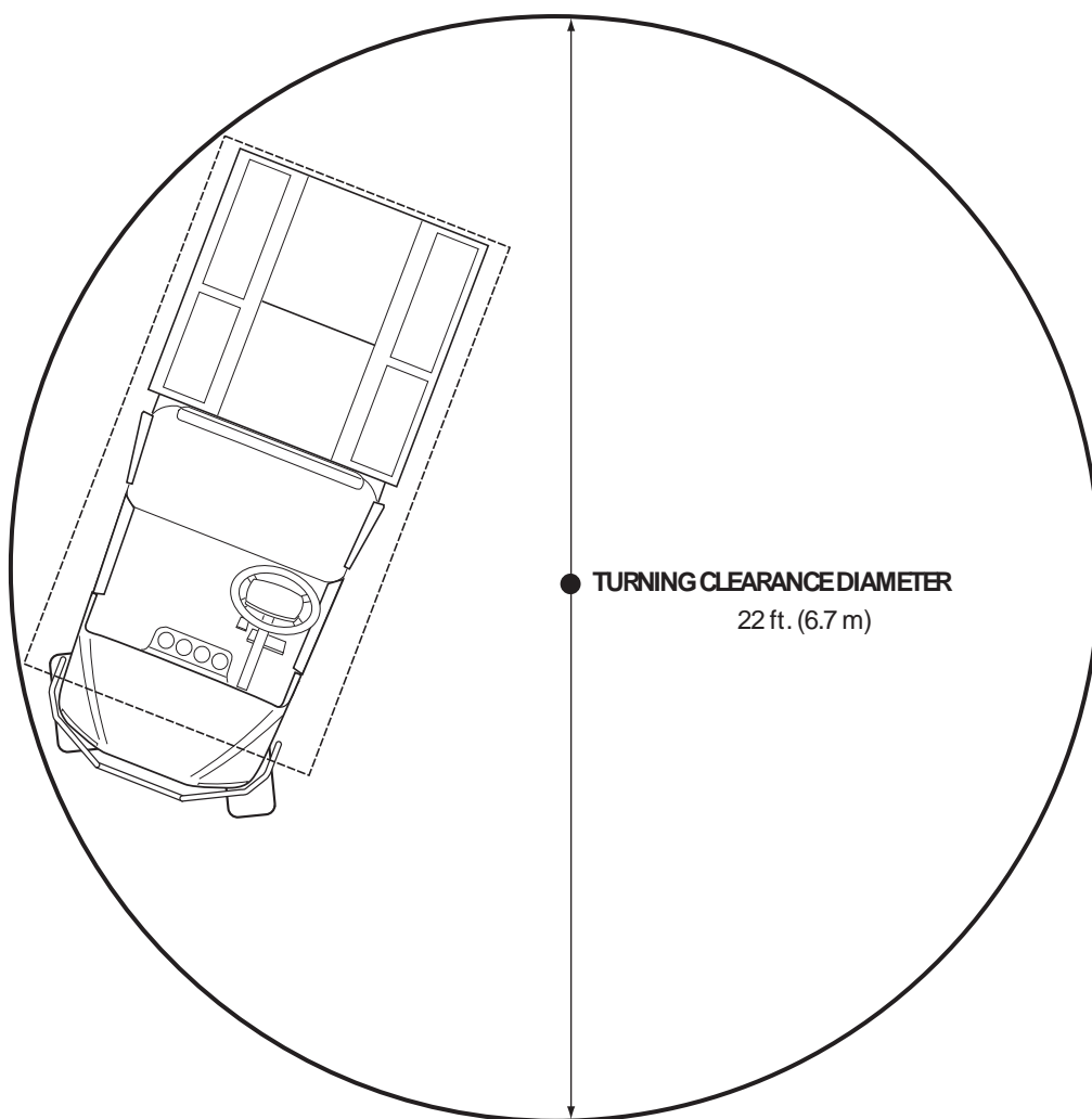
Fig. 42 Vehicle Dimensions, Incline Specifications and Turning Clearance Diameter
