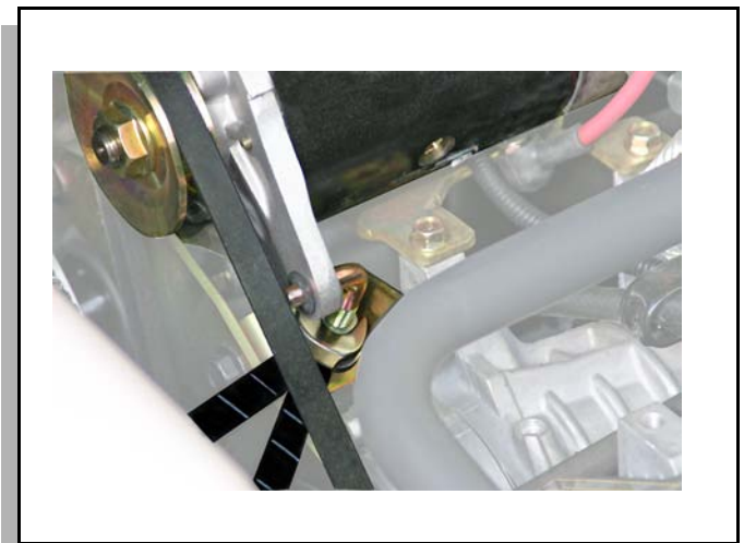
Fig. 31 Adjust Belt Tension
