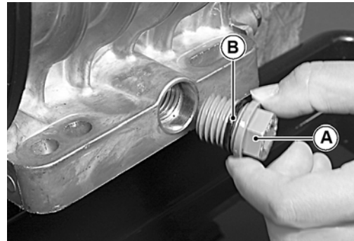
Fig. 27 Oil Drain Plug
