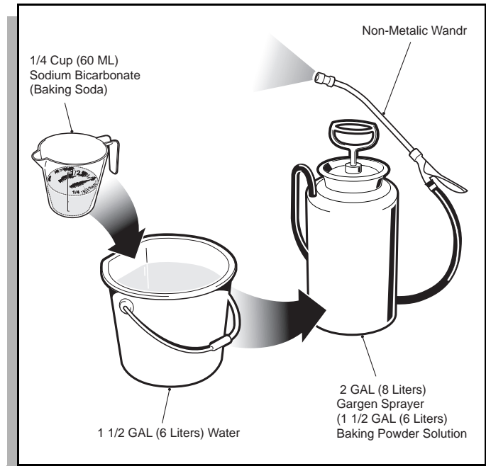
Fig. 32 Preparing Acid Neutralizing Solution
