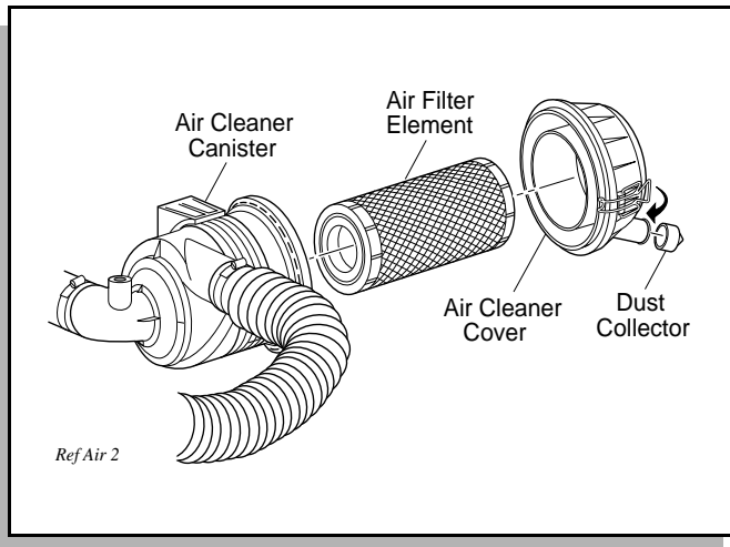
Fig. 36 Air Cleaner
