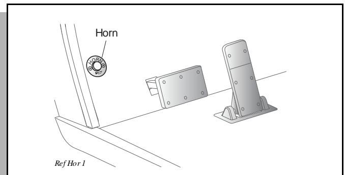
Fig. 10 Horn Button
