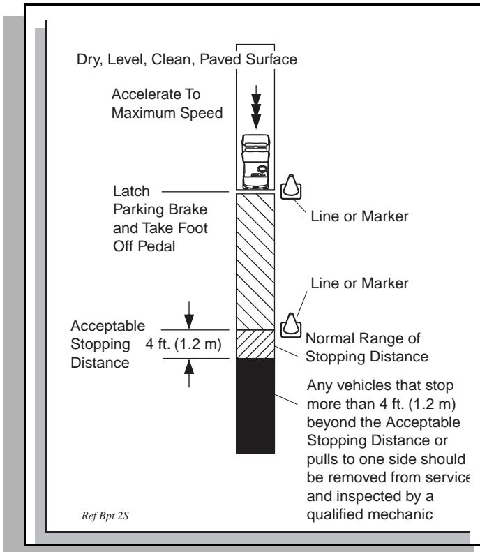
Fig. 33 Typical Brake Performance Test
