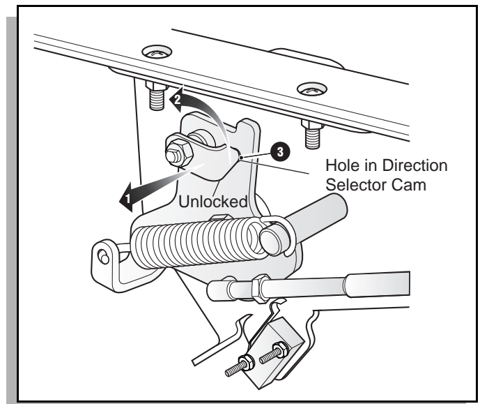
Fig. 18 Neutral Lock
