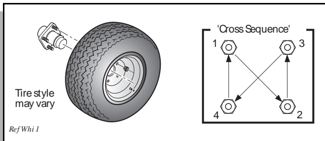
Fig. 15 Wheel Installation
