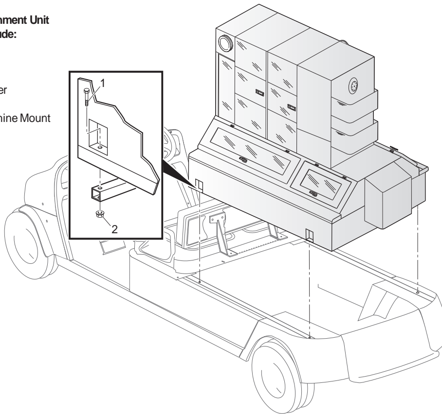
Fig. 1 Mounting the Refreshment Unit
