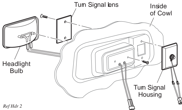
Fig. 11 Headlight and Turn Signal VEHICLE WITH A DISCHARGED BATTERY
