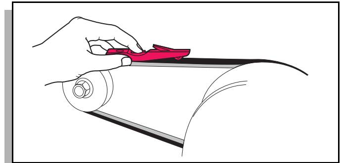
Fig. 24 Check Belt Tension with Gauge
