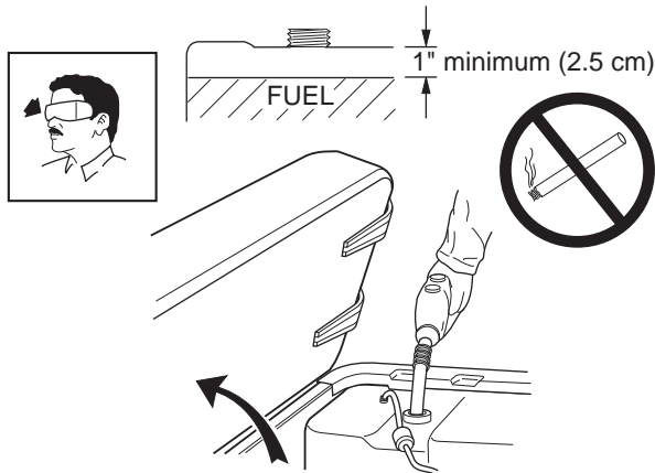
Fig. 8 Fueling
