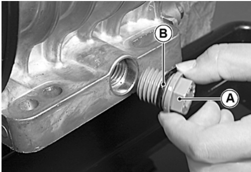
Fig. 22 Oil Drain Plug
