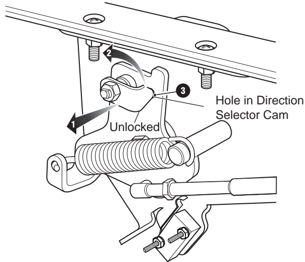
Fig. 13 Neutral Lock
