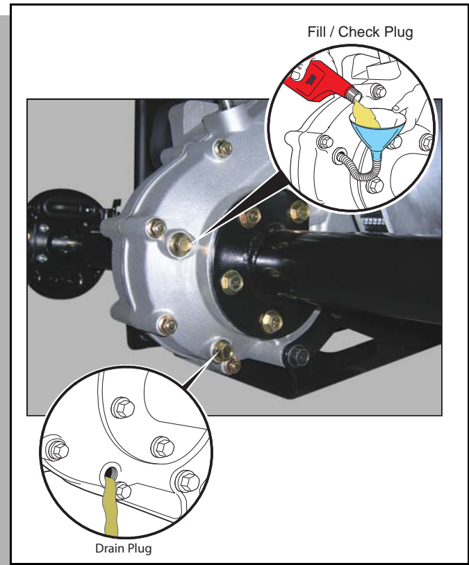
Fig. 30 Add, Check and Drain Rear Axle Lubricant is to be replaced, a drain plug is provided at the bottom of the differential housing.
