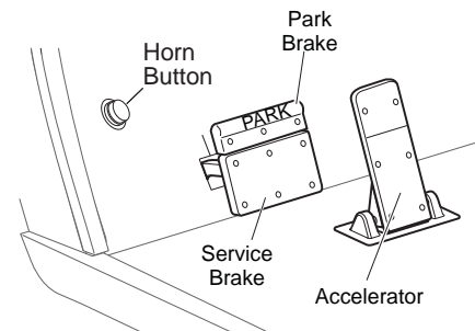
Fig. 6 Horn Button
