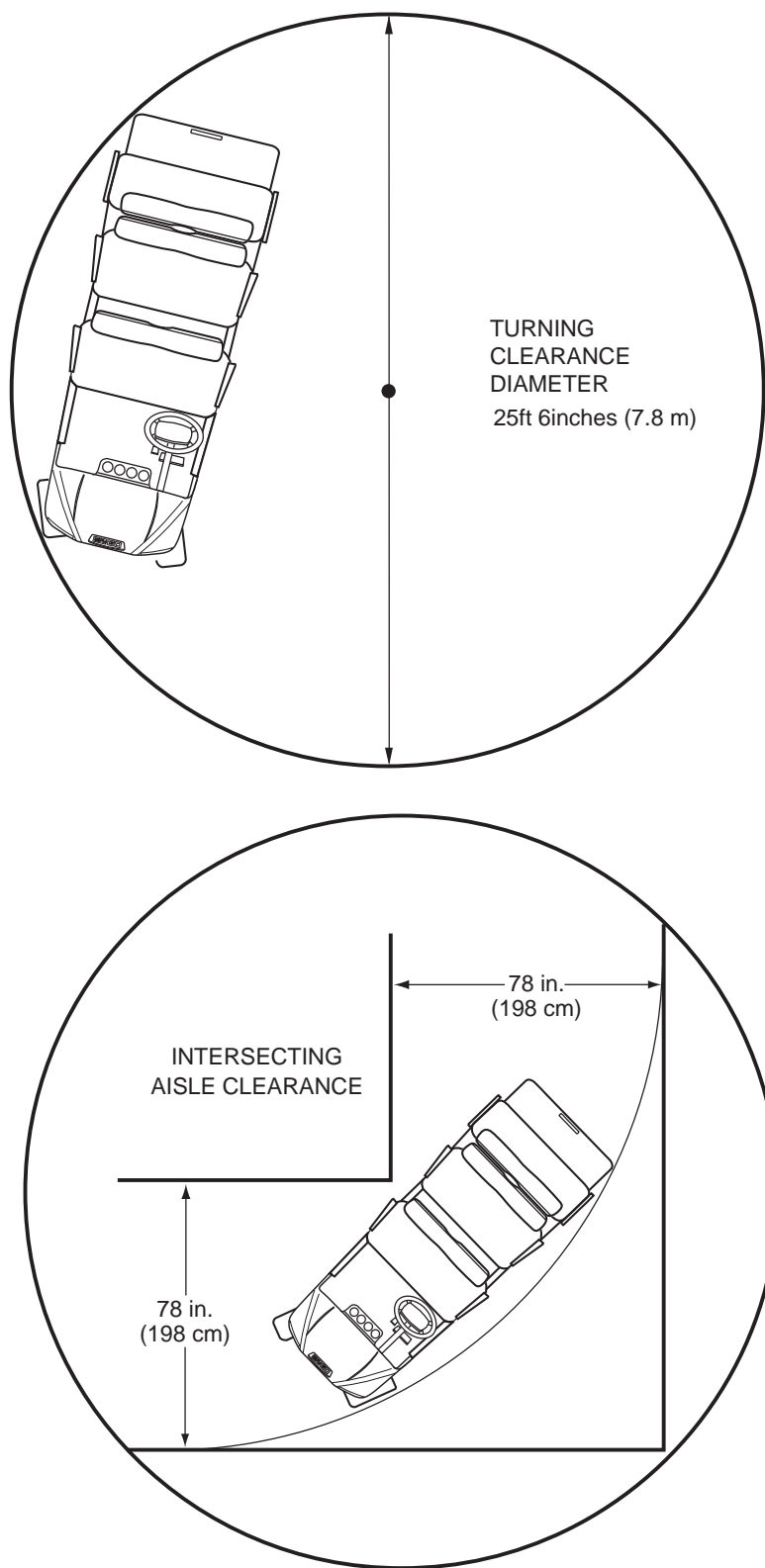
Fig. 37 Vehicle Turning Clearance
