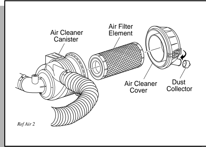
Fig. 31 Air Cleaner
