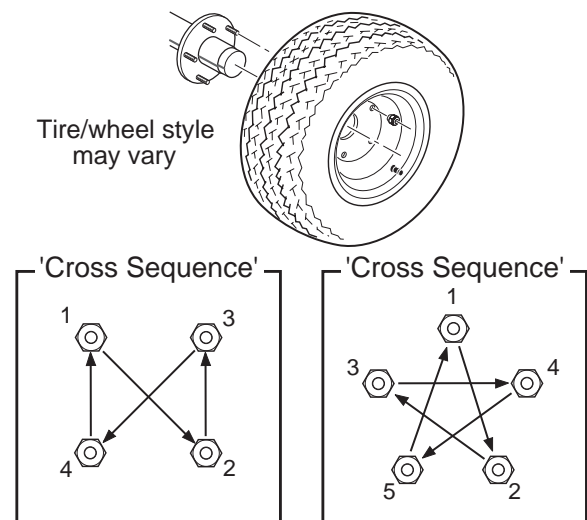
Fig. 10 Wheel Installation
