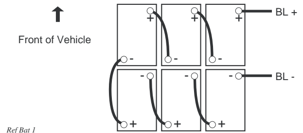
Fig. 29 36V Battery Connections
