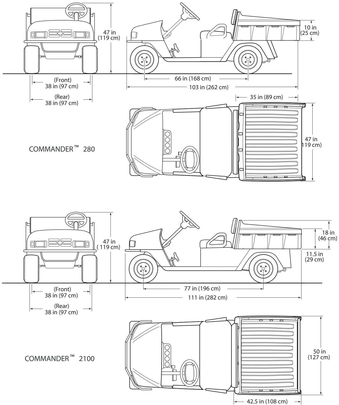
Fig. 34 Vehicle Dimensions
