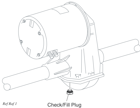
Fig. 21 Add, Check and Drain Axle Lubricant
