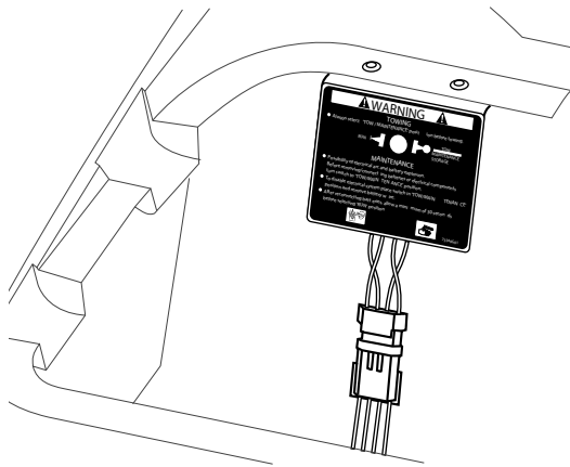
Fig. 8 Run-Tow/Maintenance/Storage Switch
