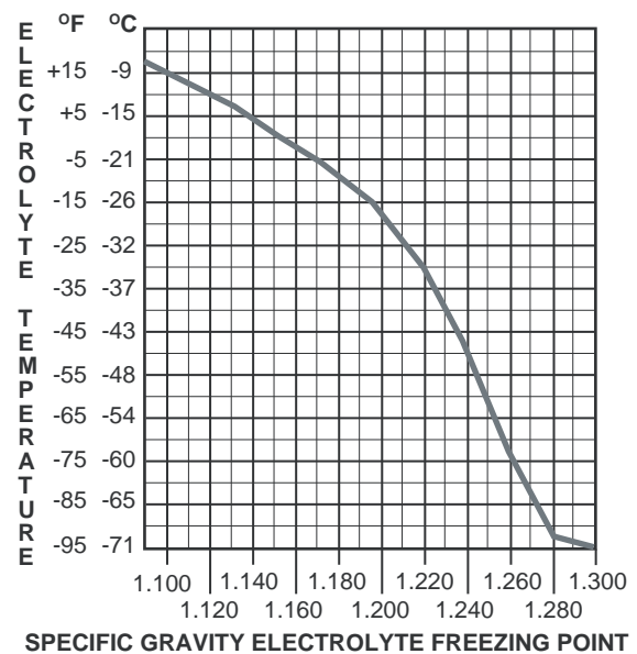
Fig. 31 Freezing Point of Electrolyte
