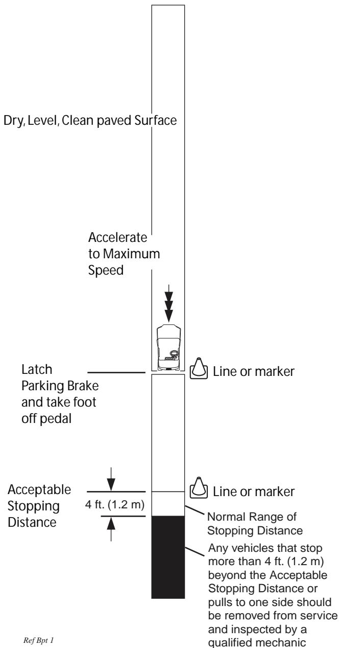
Fig. 20 Typical Brake Performance Test
