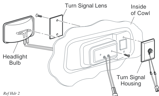
Fig. 16 Headlight and Turn Signal Bulb Replacement
