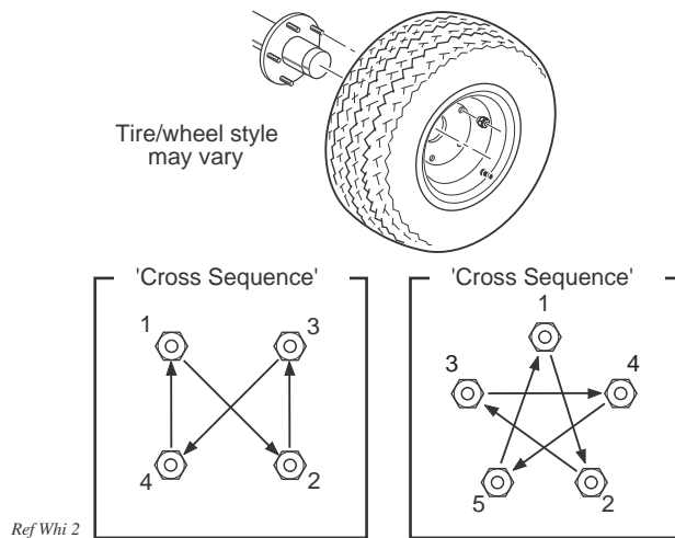
Fig. 15 Wheel Installation
