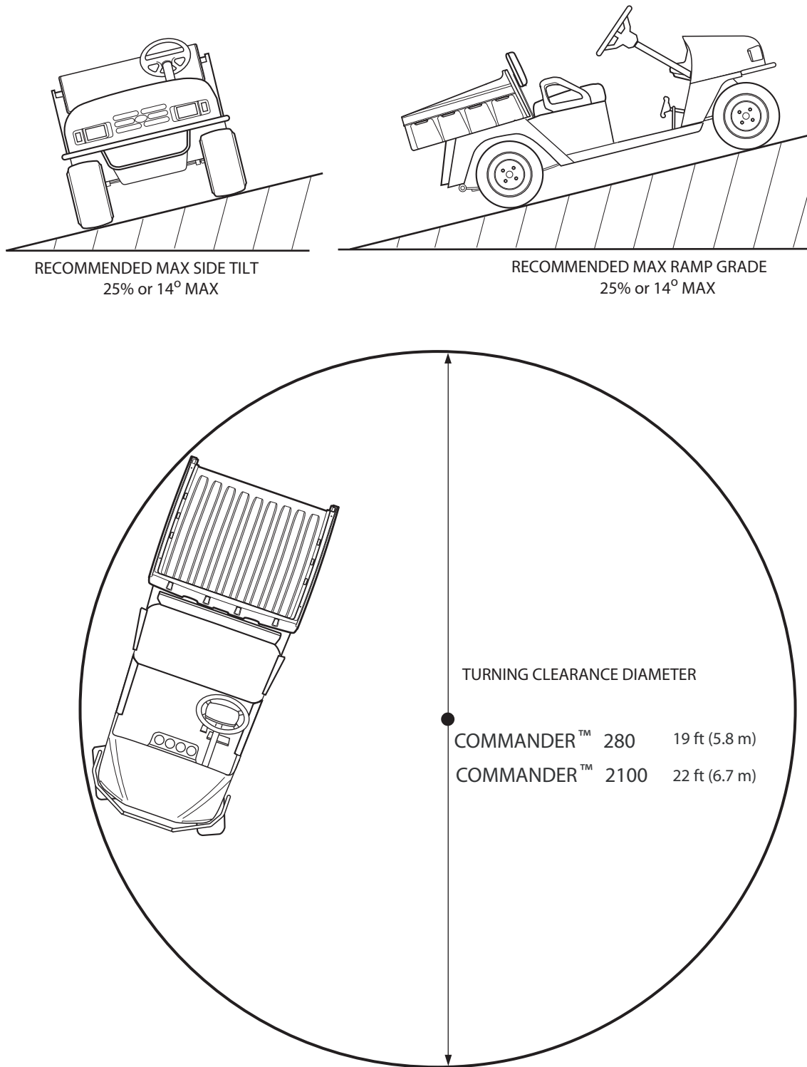
Fig. 35 Vehicle Dimensions, Incline Specifications and Turning Clearance Diameter
