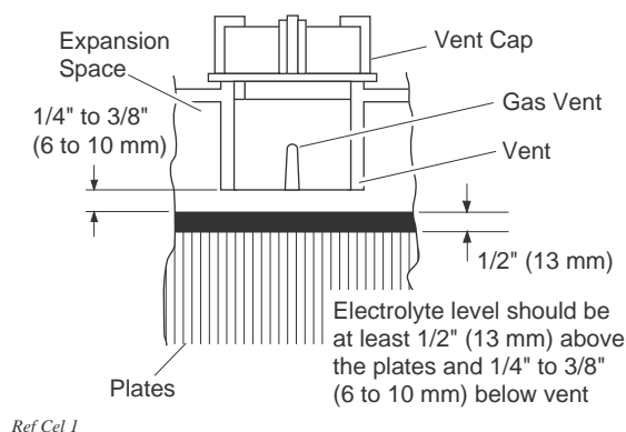
Fig. 25 Correct Electrolyte Level
