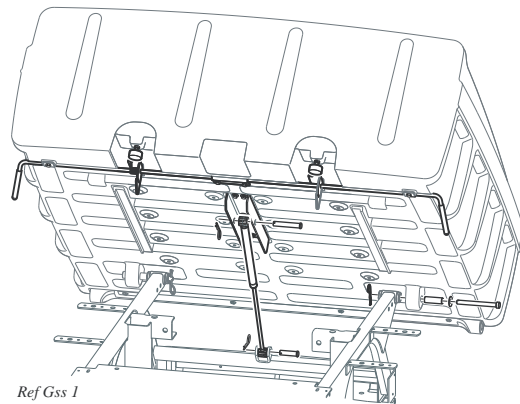
Fig. 11 Gas Strut
