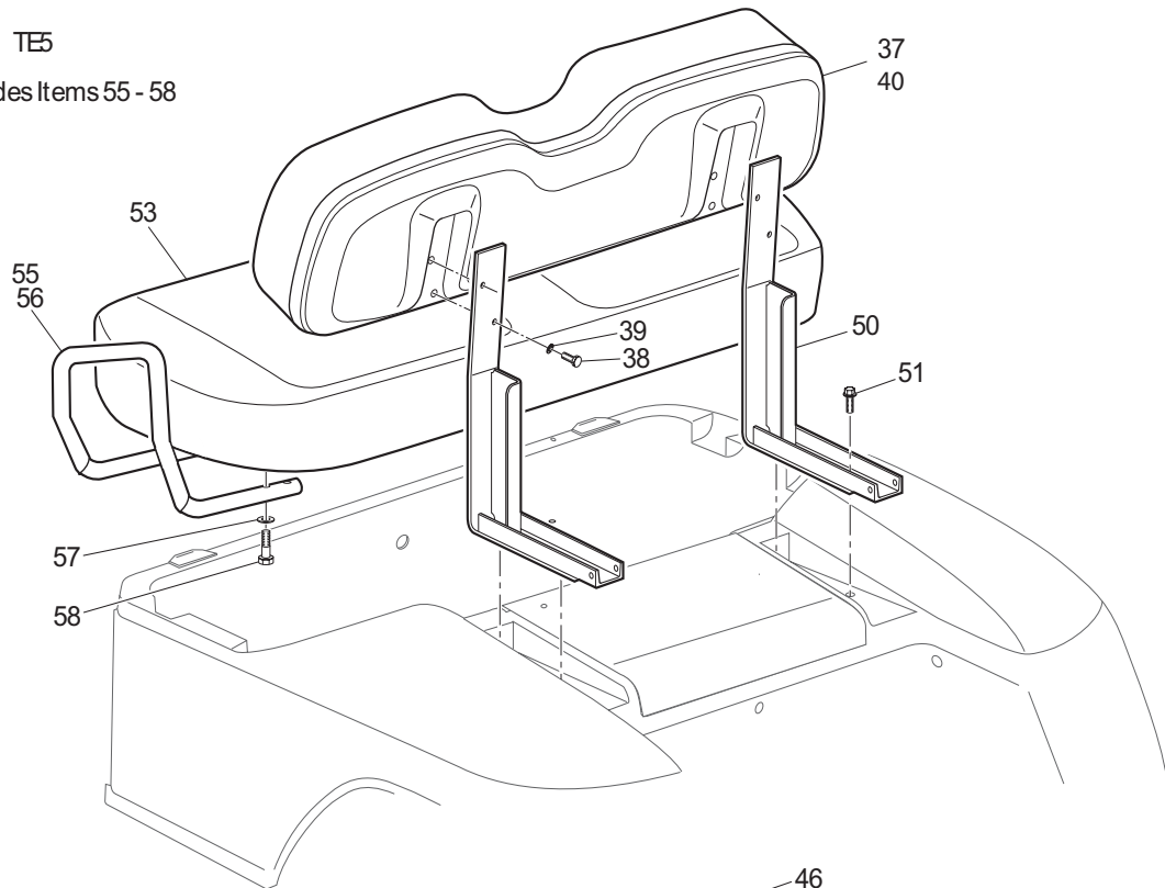
SHUTTLE 41 - Includes Items 42 - 48
